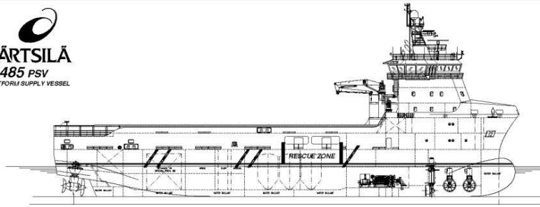
PROFILE SB
