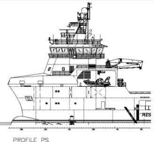
PROFILE PS
